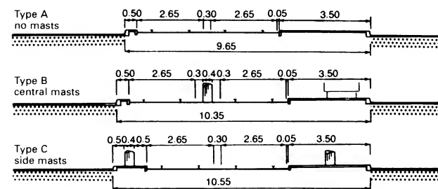
4 → 3 Tram stops on one side
